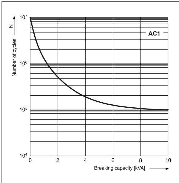
Electrical life at AC resistive load. Switching frequency: 600 cycles/hour Fig. 1
